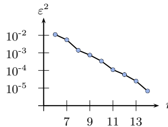
Fig. 2. Average \chi^2 and the assigned bias \varepsilon^2 for r = 6, \dots, 14 rounds (where the bias \varepsilon^2 is plotted on the right).
